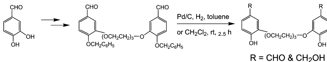
Scheme 3 DB24C8 derivatives via protection/deprotection route.
