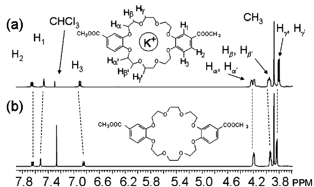
Fig. 1 400 MHz 1 H NMR spectra in CDCl 3 : (a) crude product before washing with water, 1 \cdot K^+ PF_6^- , (b) crude product after washing with water, 1 .
